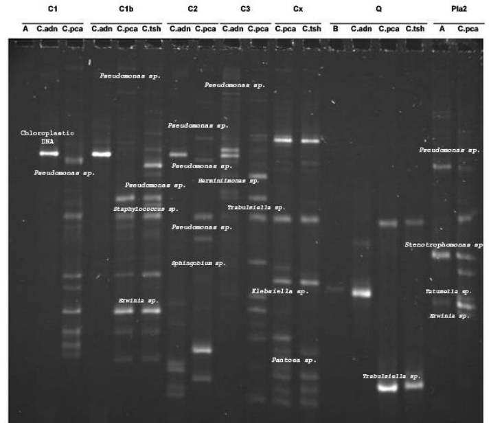
Figure 3 Bacterial 16S rDNA PCR-TTGE profiles obtained from pollen samples of Cupressus (C1, C1b, C2 and C3), Cephalotaxus (Cx), Quercus (Q) and Platanus (Pla2) prepared according to five protocols (A, B, C.adn, C.pca, C.tsh).
