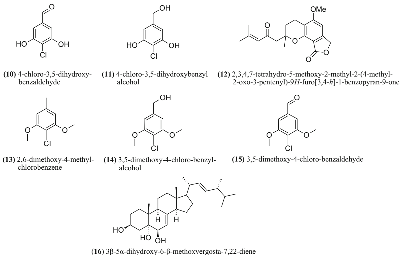
Fig. 4 Chemical structures of chlorinated aromatic compounds, benzopyrans, benzofurans and an ergosterol derivative isolated from Hericium erinaceus
